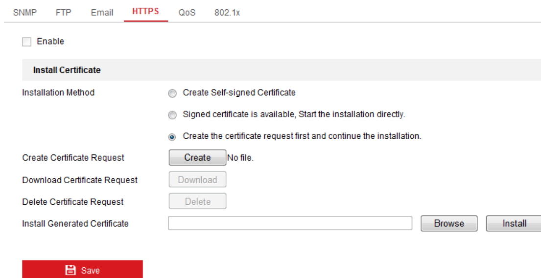
Figure 5-29 HTTPS Settings
