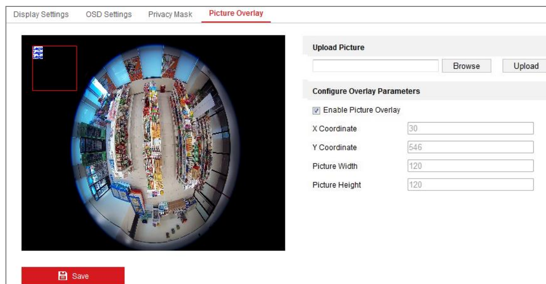
Figure 5-42 Picture Overlay
