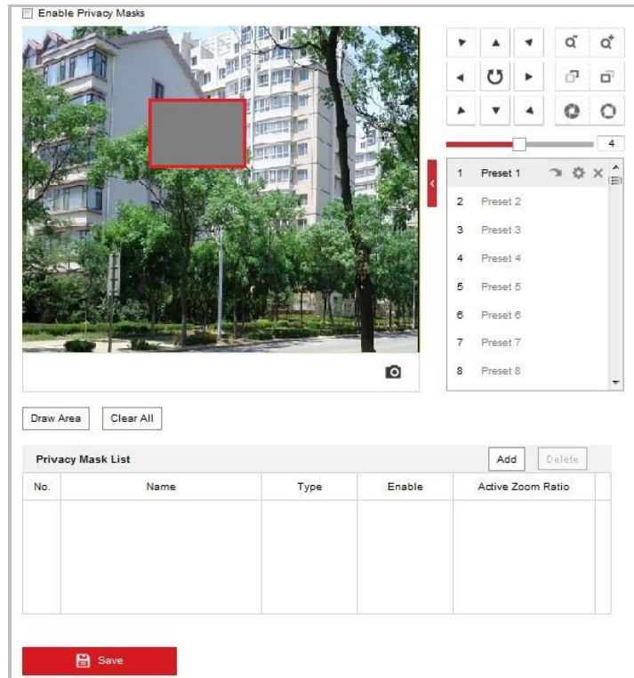
Figure 5-30 Draw the Privacy Mask
