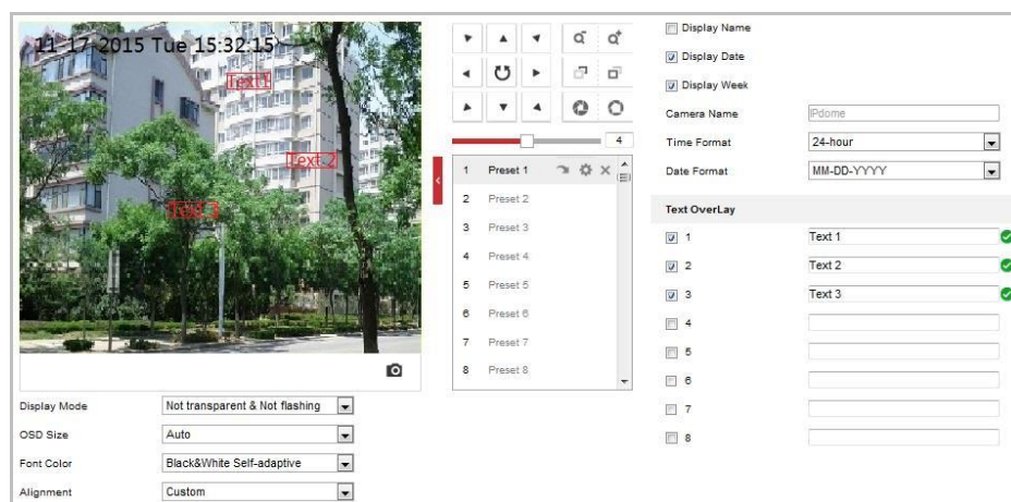
Figure 6-37 Text Overlay Settings
