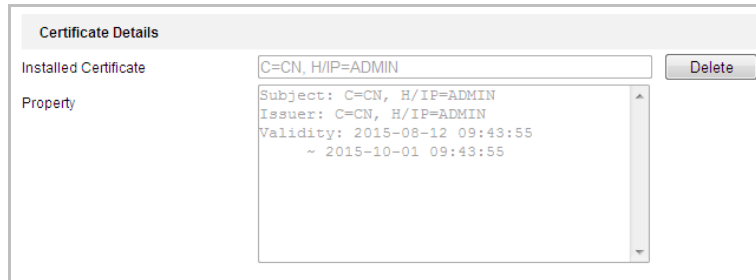
Figure 6-17 Installed Certificate Property
