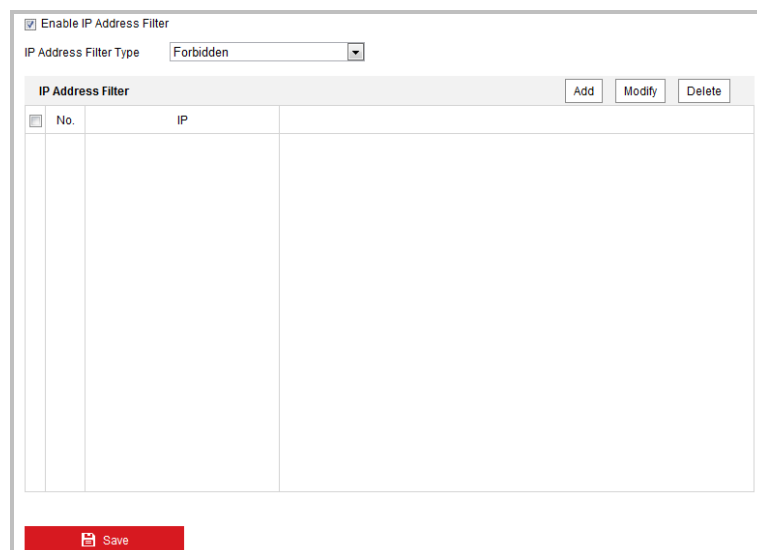
Figure 6-50 IP Address Filter
