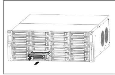
Figure 2-8 Push HDD Case into Slot
