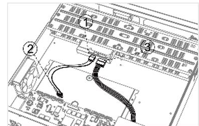
Figure 2-3 Connect Cable
