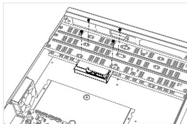
Figure 2-2 Fix HDD
