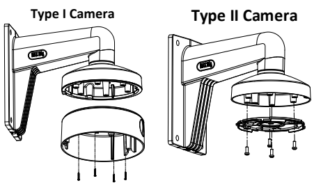
Figure 2-6 Attach the Base Plate to the Mount
