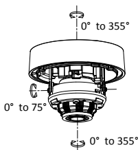
Figure 2-10 3-Axis Adjustment
