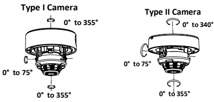
Figure 2-4 3-Axis Adjustment
