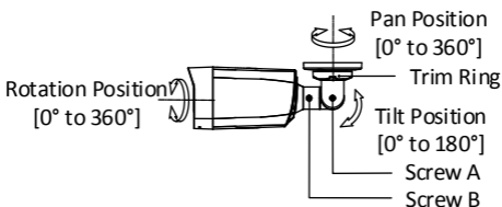
Figure 2-2 3-Axis Adjustment
